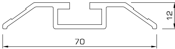
101 - Threshold rail with single channel
